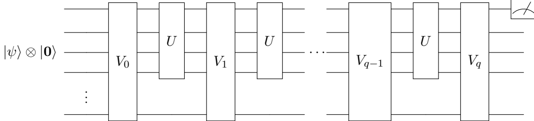
Figure 2: Schematic of a QMAP protocol that receives a proof state |\psi\rangle and makes q queries to a unitary U .
